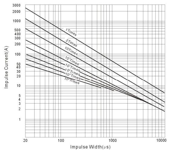
Surge Life Time Reting [820LD10 to 112KD10]
