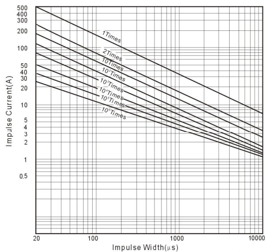
Surge Life Time Reting [180LD10 to 680KD10]
