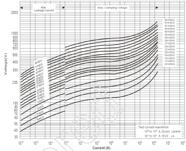
V-I Curve [820KD10 to 561KD10]
